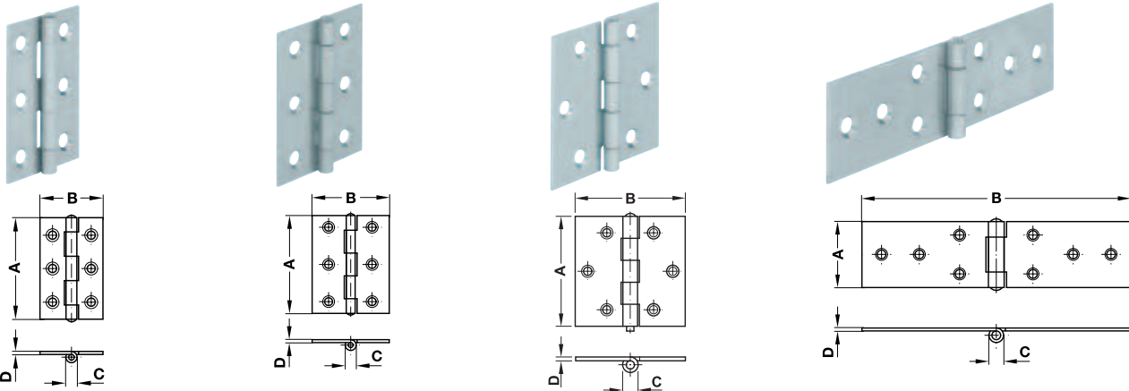
Narrow, in compliance with DIN 7954
