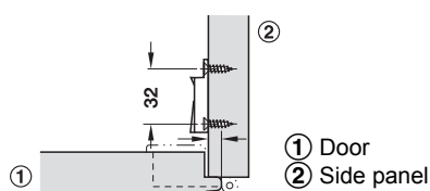
Overlay 5 mm with mounting plate 0 mm
