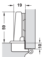
With mounting plate distance 0 mm
