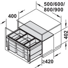
Three compartment waste bin
