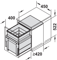
Single waste bin
