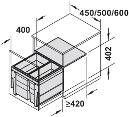
Two compartment waste bin
