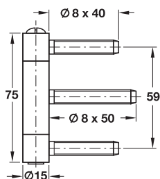
BAKA C 1-15 WF for blind frames
