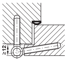
BAKA C 1-15 WF for blind frames
