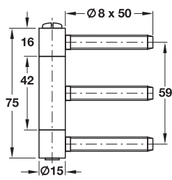
BAKA C 2-15 WF for lining frames
