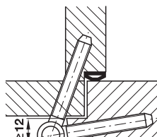
BAKA C 2-15 WF for lining frames
