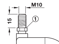
Threaded pin, steel, galvanized ① Hexagon nut SW13
