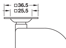
Screw-on plate, steel, galvanized
