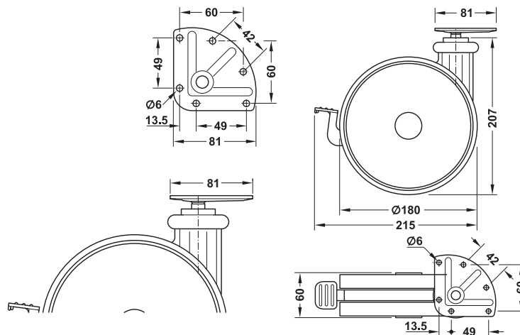
With screw-on plate, steel, galvanized Free running, with brake
