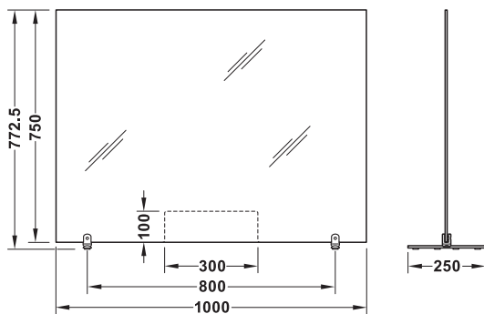
With cut-out
