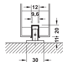
Clear threshold floor guide with guide track
