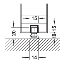
Floor guide with U-shaped guide track and floor guide roller
