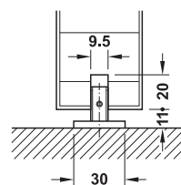
Clear threshold floor guide without guide track
