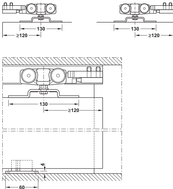
Section trolley hanger and guide
