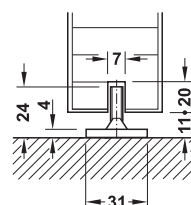
Floor guide without guide track
