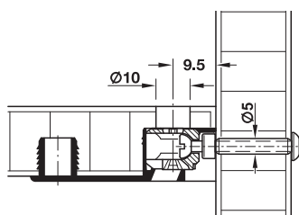
One-sided installation
