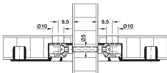
Double-sided installation
