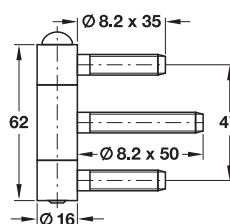
Herkula 316 GL-RA for blind frames
