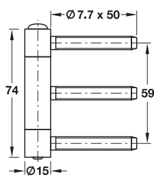
Herkula 315 GL-FR for lining frames
