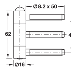
Herkula 316 GL-FR for lining frames
