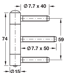
Herkula 315 GL-RA for blind frames
